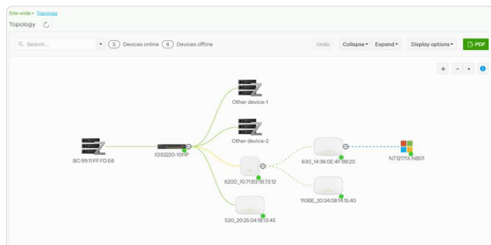
Site-wide topology with wired and wireless clients
