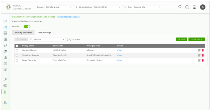
User Privilege Policy Management
