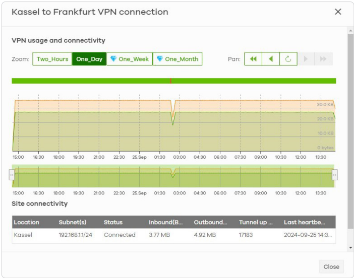
VPN usage and connectivity histogram
