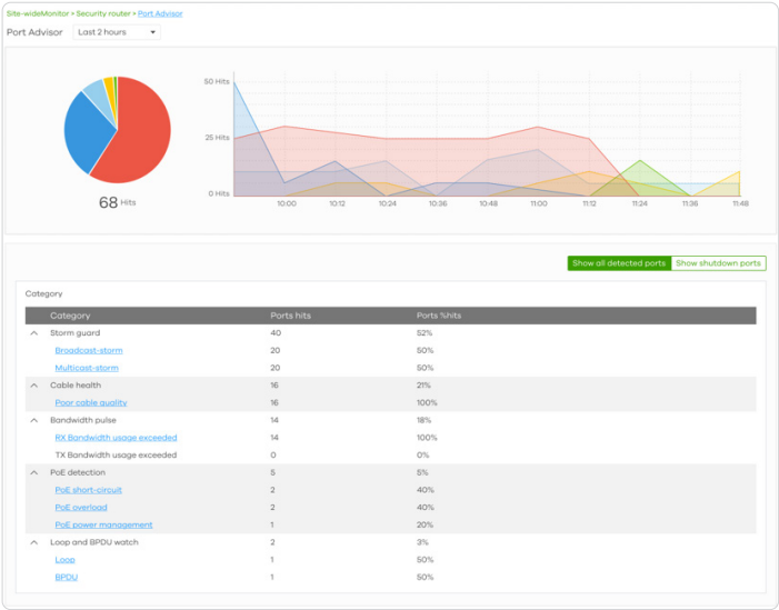
Port abnormal issue summary and analysis
