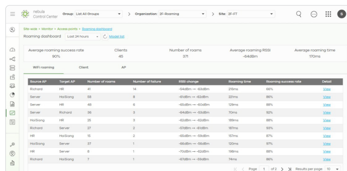
Roaming Dashboard – WiFi roaming overview
