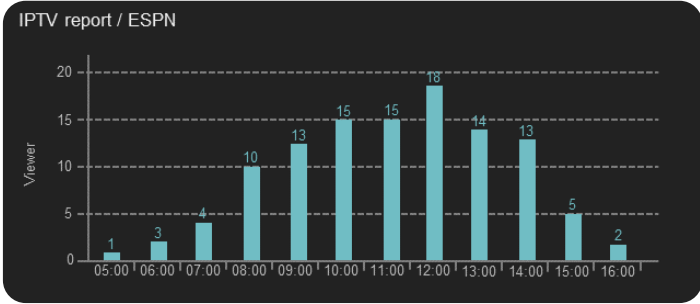
Identifies peak viewership rate for each channel
