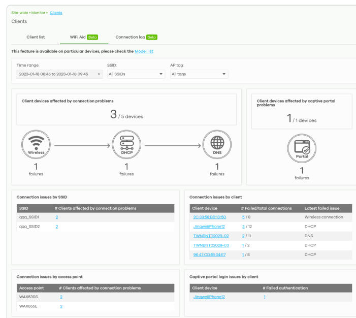
WiFi Aid – Connection failure summary and issue diagnosis
